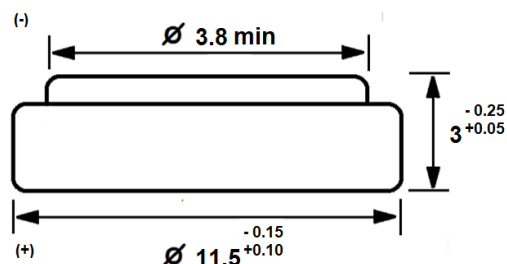
Dimensions are in millimetres
